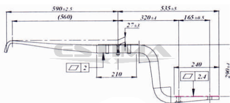
Ref. no.: 36R0702E resor/spring/peccopa/pecopa
